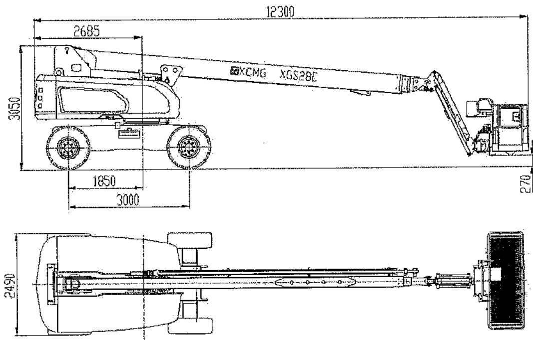
Fig. 10-1: Overview of dimensions
