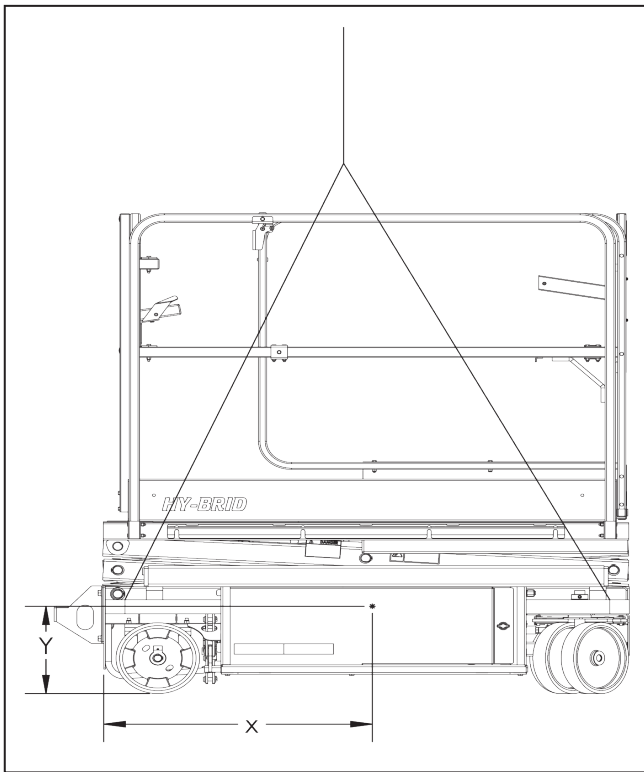
FIGURE 10: Center of Gravity
