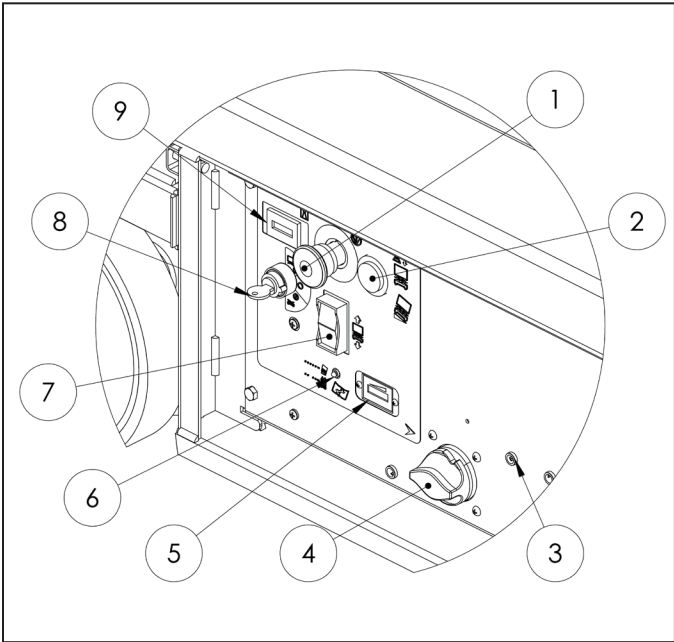
FIGURE 11: Base Controls
