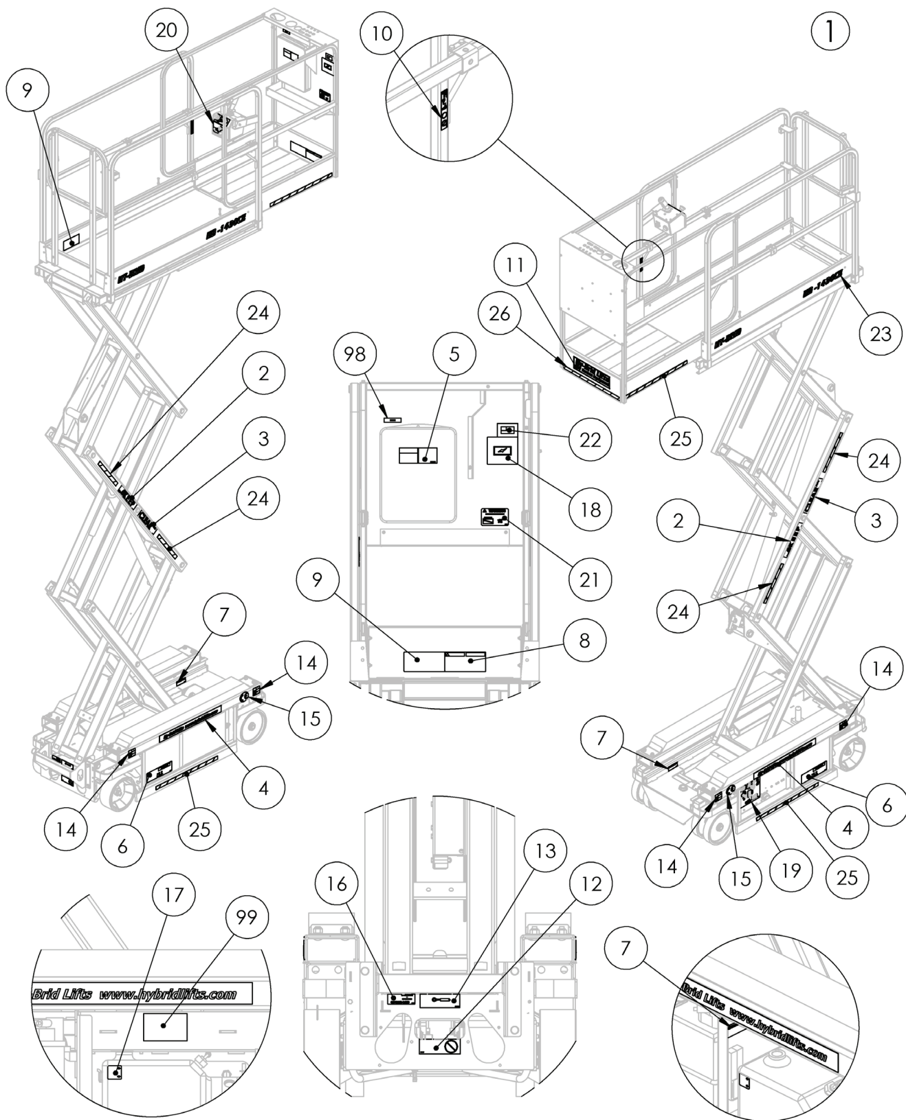
FIGURE 6: Decal Locations
