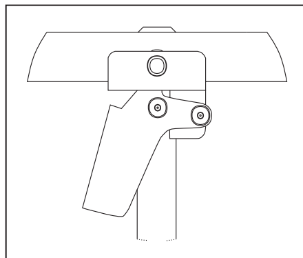
FIGURE 17: Slide Brake
