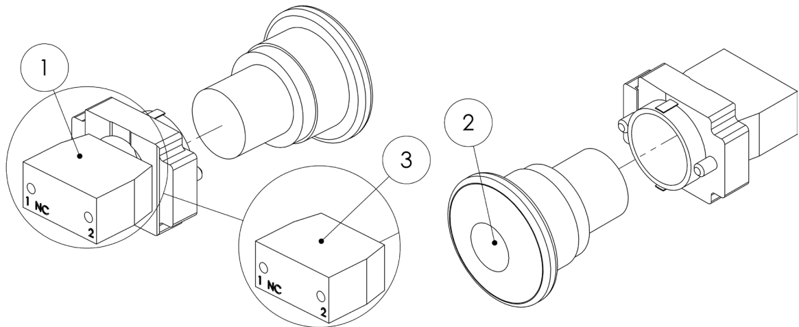
FIGURE 9: E-Stop Switch Subparts
