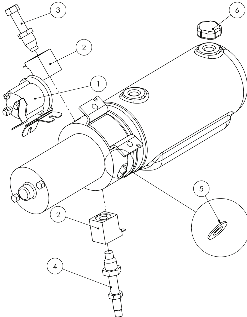
FIGURE 4: Pump Subparts
