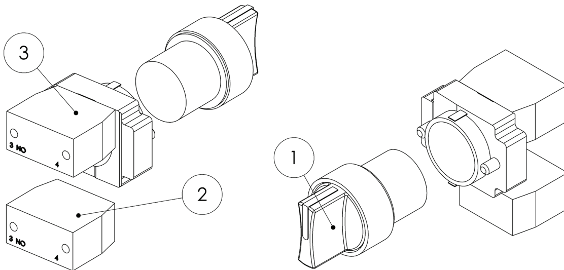
FIGURE 11: Up/Down Switch Subparts
