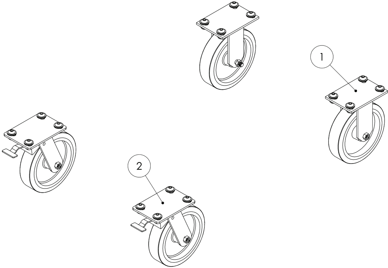
FIGURE 1: Caster Parts
