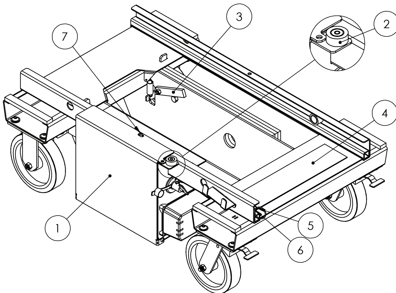
FIGURE 5: Miscellaneous Base Parts
