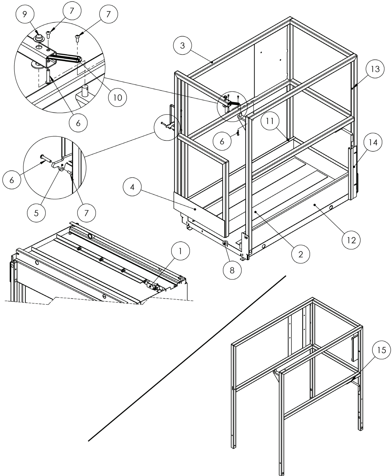
FIGURE 14: Platform & Rails
