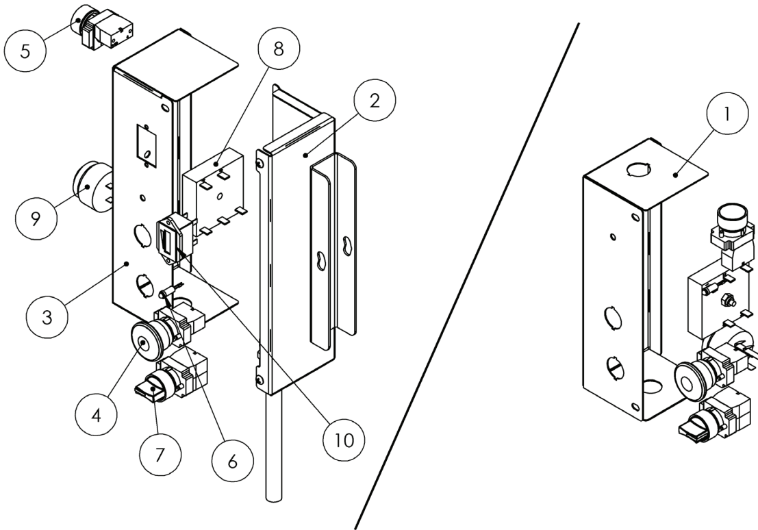
FIGURE 7: Upper Control Parts
